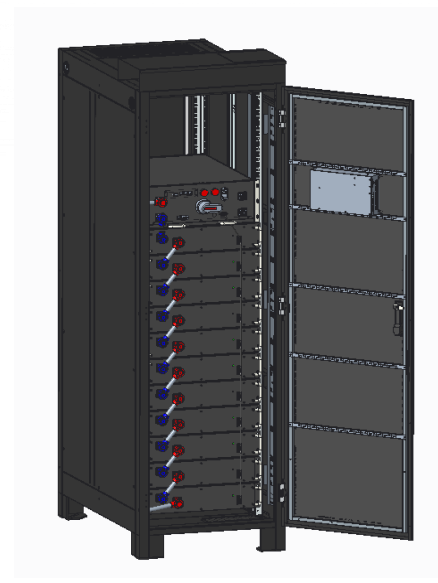
Rack 563.2V100Ah
