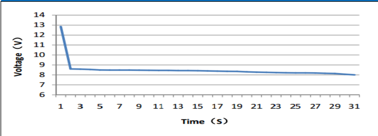
Cold Cranking Test Graph (-18°C, 950CCA)
