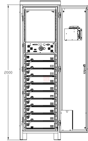
Cabinet TPL50
