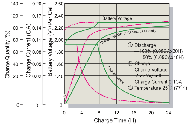
Figure 2 Charging Characteristics
