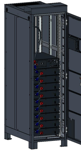
Rack 460.8V100Ah
